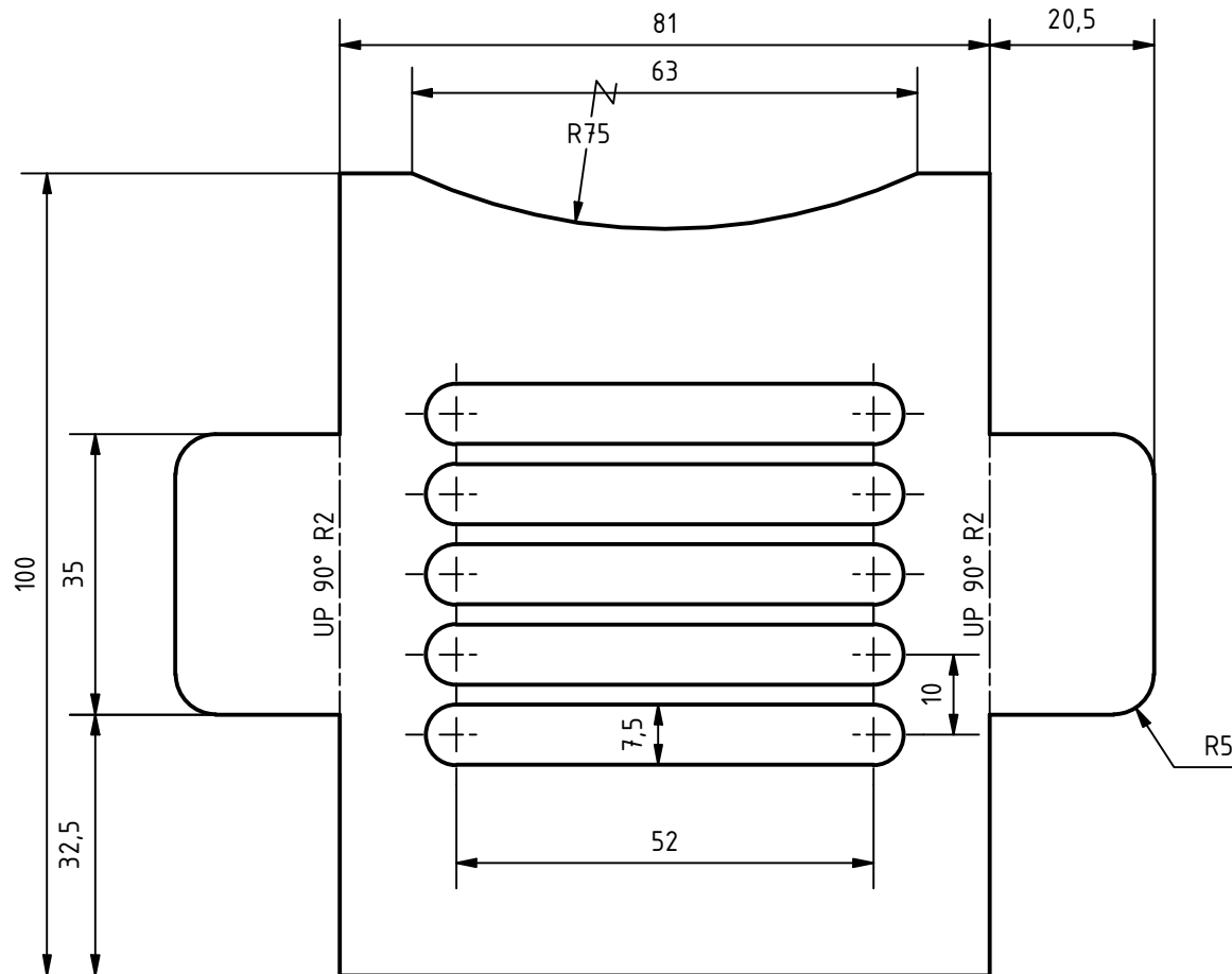
flat pattern
