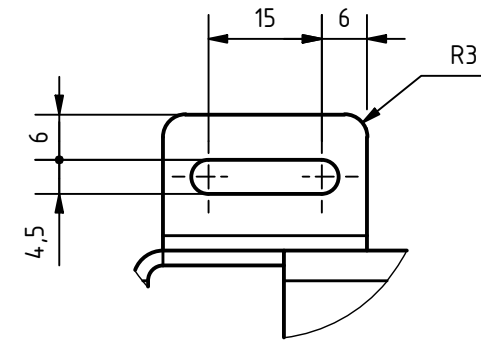
Detail A (1 : 1)
